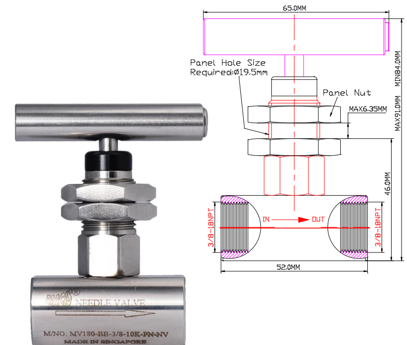
Ordering Ref : MV 180-BB-3/8-10K-PN-NV-L
