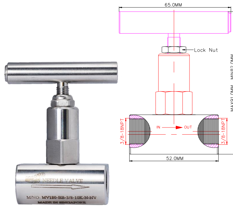
Ordering Ref : MV 180-BB-3/8-10K-N-NV-L
