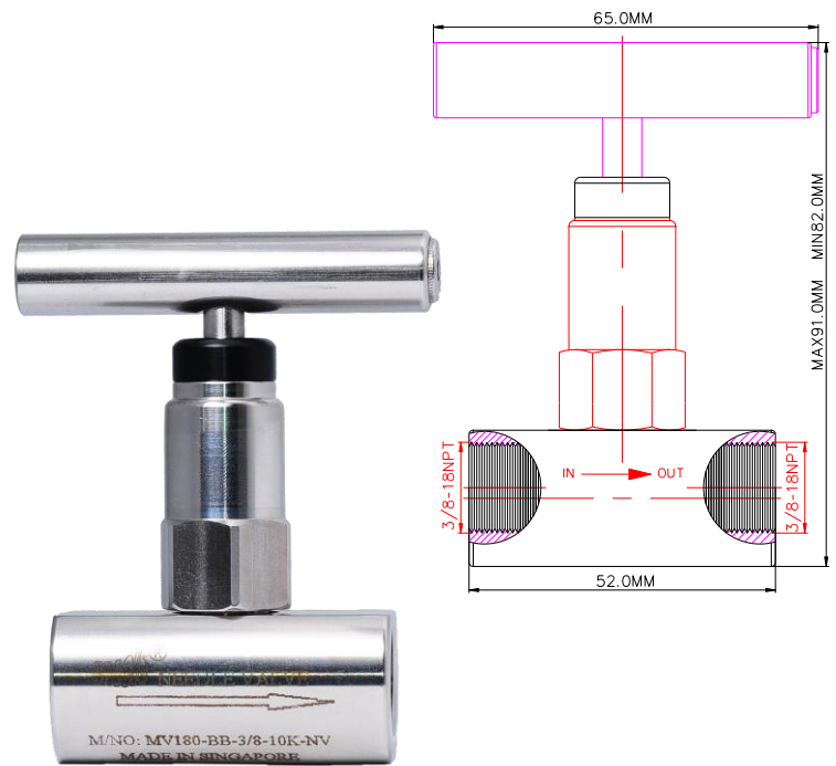
Ordering Ref : MV 180-BB-3/8-10K-NV-L
